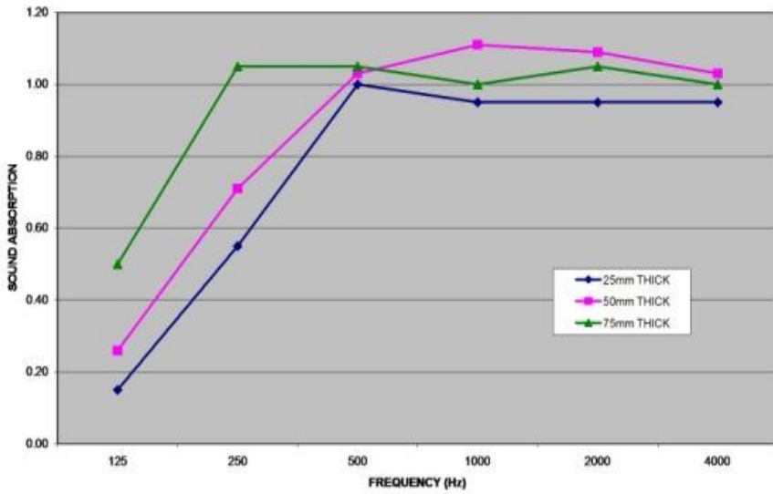
SERENITY ACOUSTIC PANELS - SOUND ABSORPTION COMPARISON AT VARIOUS THICKNESSES
